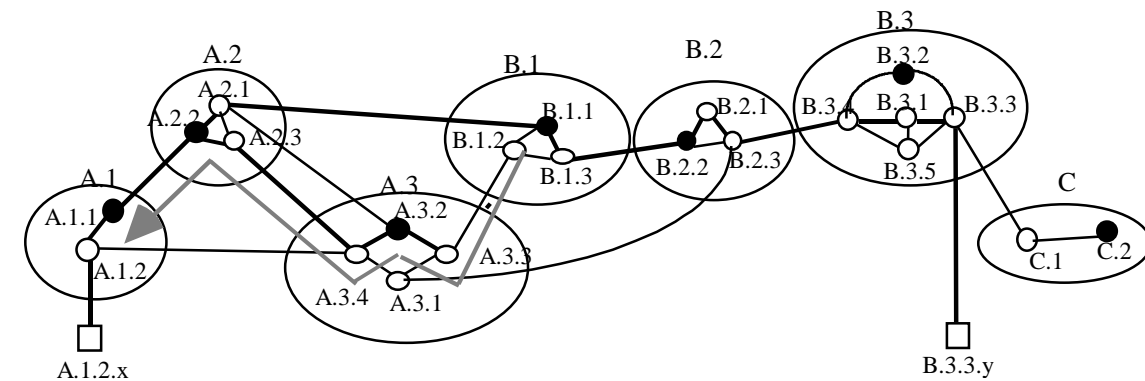
Figure 4-4: An Example of Explicitly Routed Call
