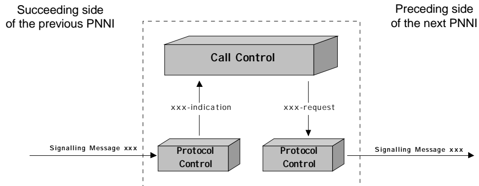
Figure 6-1a: Primitives used in the Signalling specification sections
