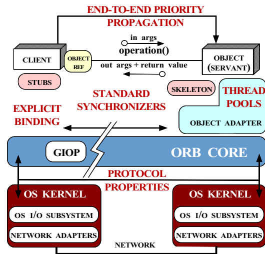
Figure 1: Standard Capabilities in Real-time CORBA ORB Endsistemas
