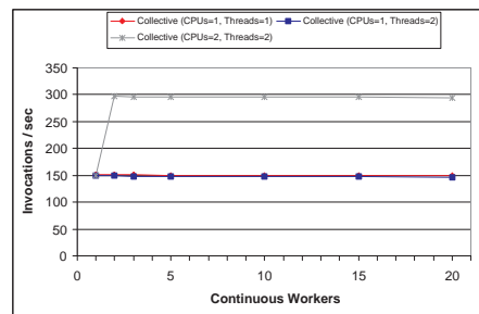
Figure 13: Effect of Increasing Concurrency
