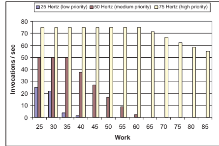
Figure 30: Effect of Increasing Workload in Real-time CORBA without Lanes: Server Thread Pool Priority = High
