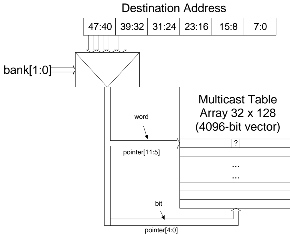
Figure 13-2. Multicast Table Array
