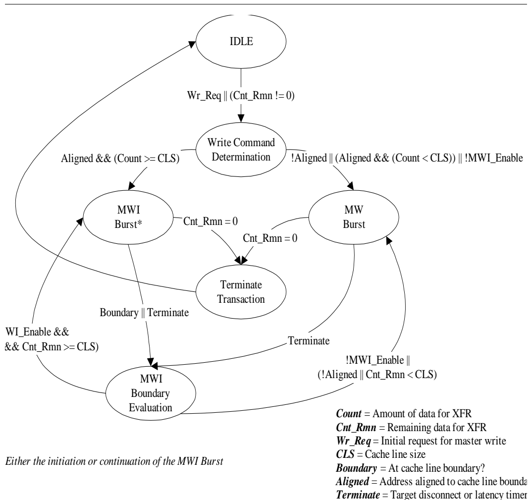
Figure 4-4. Master Write Command Usage Algorithm
